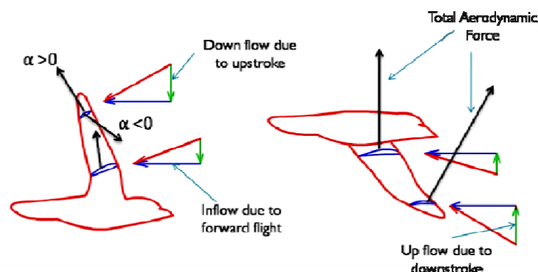
Figure 12. Forces Generated During Upstroke and Down stroke
