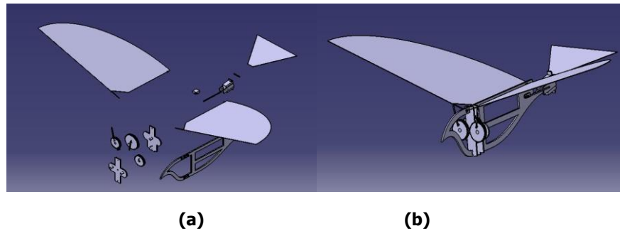
Figure 11. (a) Sub components of final assembly; (b) CAD Model of final assembly
