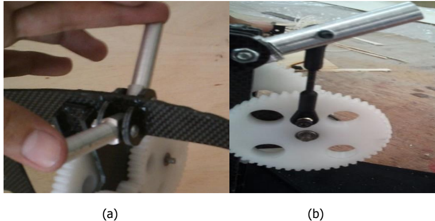
Figure 33. Drive linkages. (a). Wing connectors; (b) Main drive linkage
