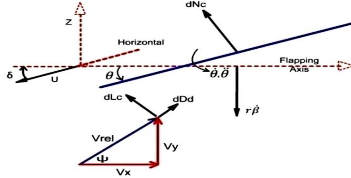
Figure 18. Forces on Each Section of Wing
