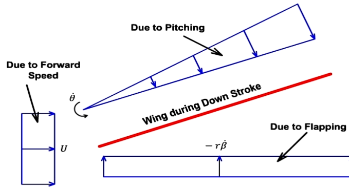
Figure 17. Relative Air Flow
