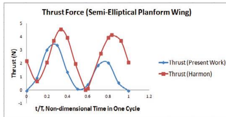
Figure 26. Thrust Force (Present Work Vs Harjino [35])
