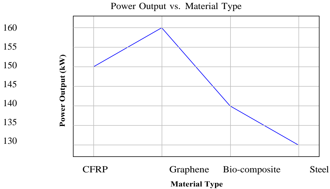
Figure-1 Comparison of power output for different materials.
